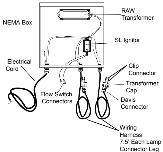
Viper 400 Trans 208/230/240V-60Hz
