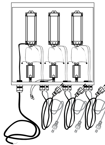
Viper 1200 Trans 208/230/240V-60Hz
